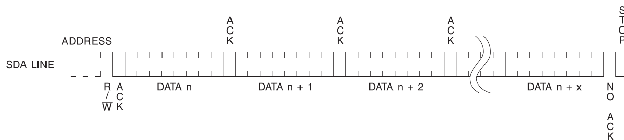
Figure 10. Sequential Read
